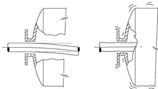
Shaft Deflection
