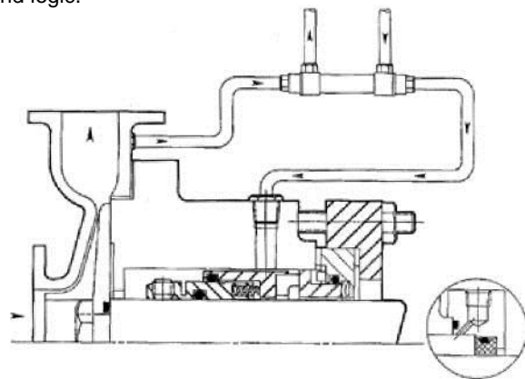
Figure 32 - Recirculation Discharge Return
