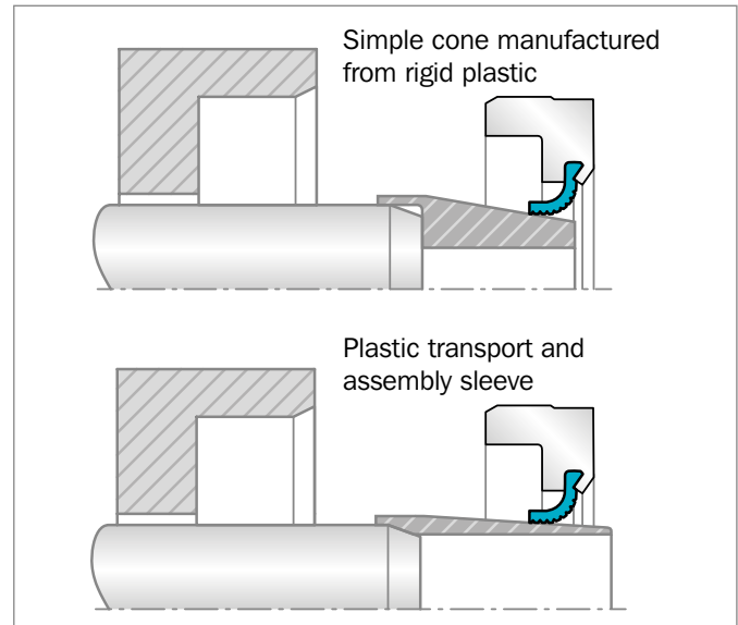
Figure 16: Assembly tooling types for installation on shafts
