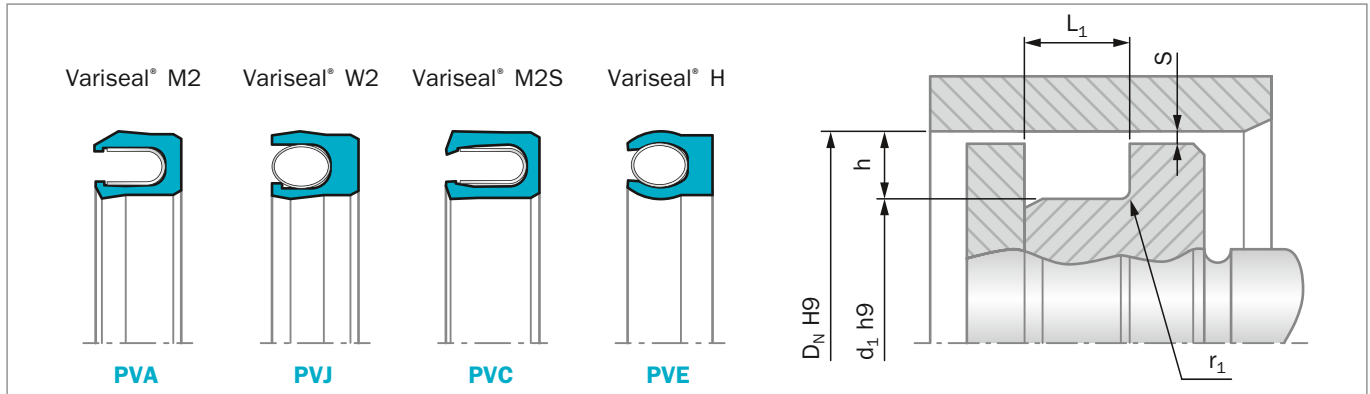
Figure 22: Installation Drawing
