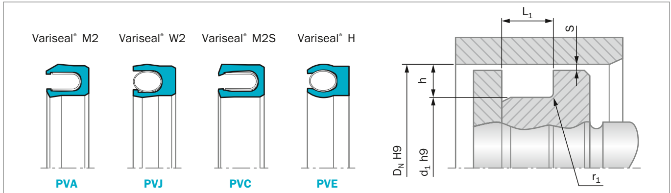
Figure 21: Installation Drawing
