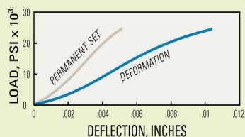
Figure E Deflection
