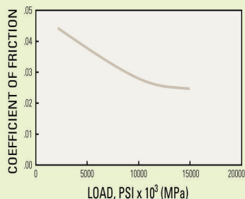
Figure F Coefficient of Friction vs. Load for FCJ Bearing
