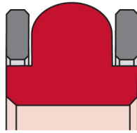
Seal Profile: DK120
