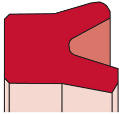
Seal Profile: DK105
