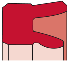
Seal Profile: DS205
