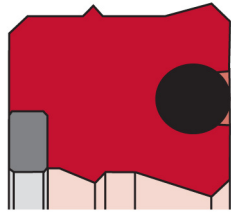
Seal Profile: DS131A
