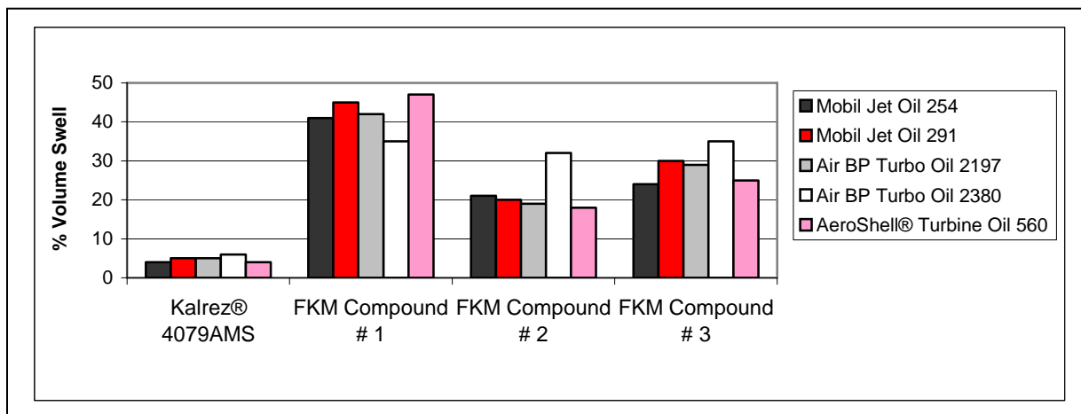
Figure 1 Long-Term Volume Swell In Standard* & HTS** Gas Turbine Engine Lubricating Oils 1 1008 hours at 232°C (450°F) – Oil Changed Weekly 2
