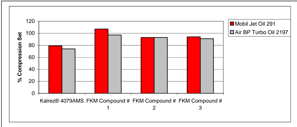
Figure 2 -- Long-Term Compression Set In HTS* Gas Turbine Engine Lubricating Oils 1 1008 Hours at 232°C (450°F) - Oil Changed Weekly 2
